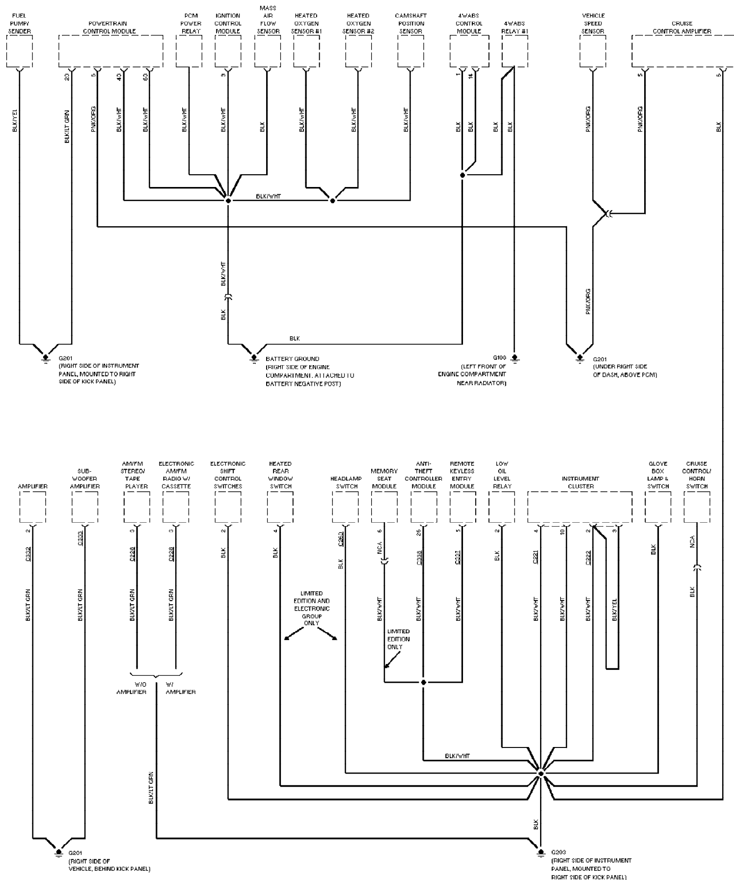
Fig. 12: Ground Distribution Circuit (2 of 3) 1994 Ford Explorer
