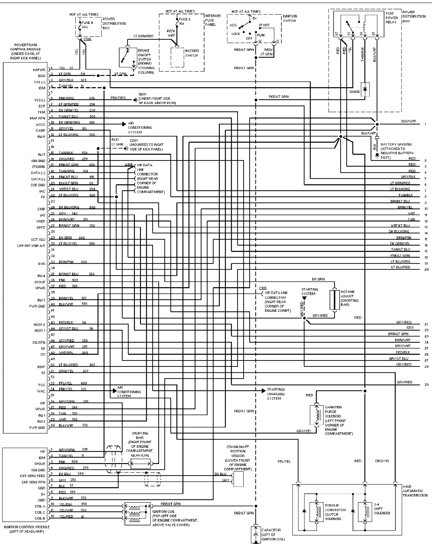
Fig. 6: 4.0L, Engine Performance Circuits (1 of 2) 1994 Ford Explorer
