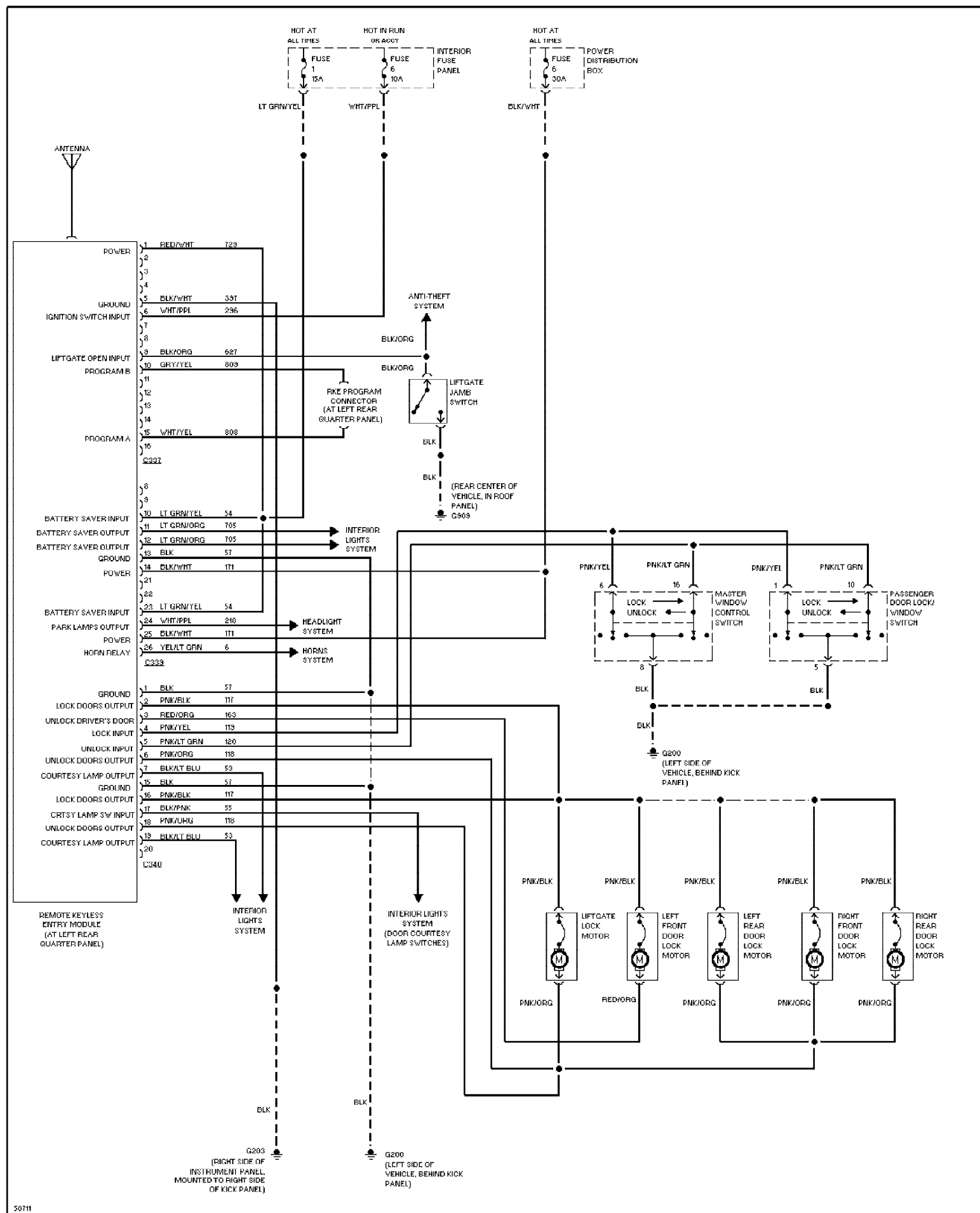
Fig. 31: Keyless Entry Circuit 1994 Ford Explorer
