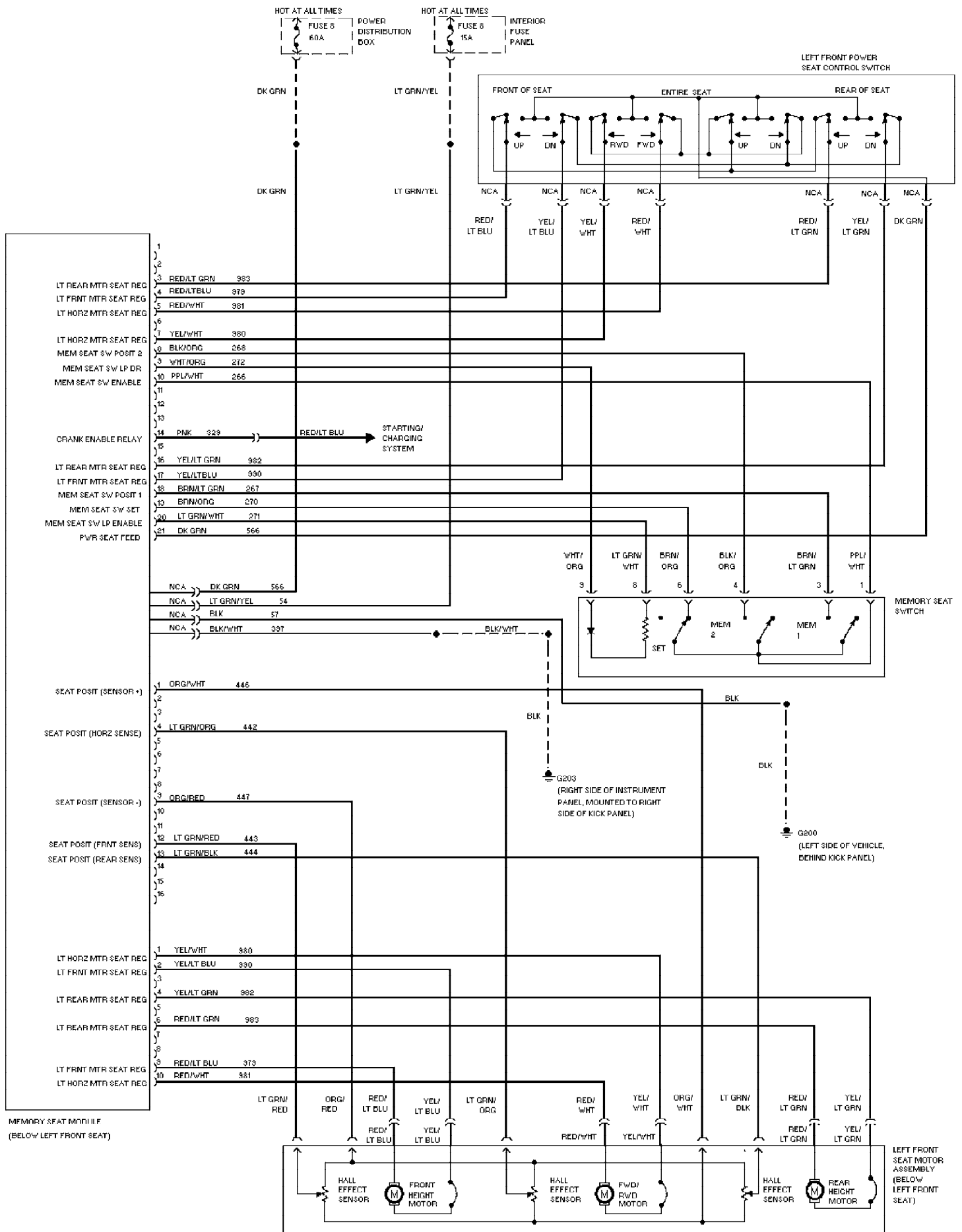
Fig. 37: Memory Seat Circuit 1994 Ford Explorer
