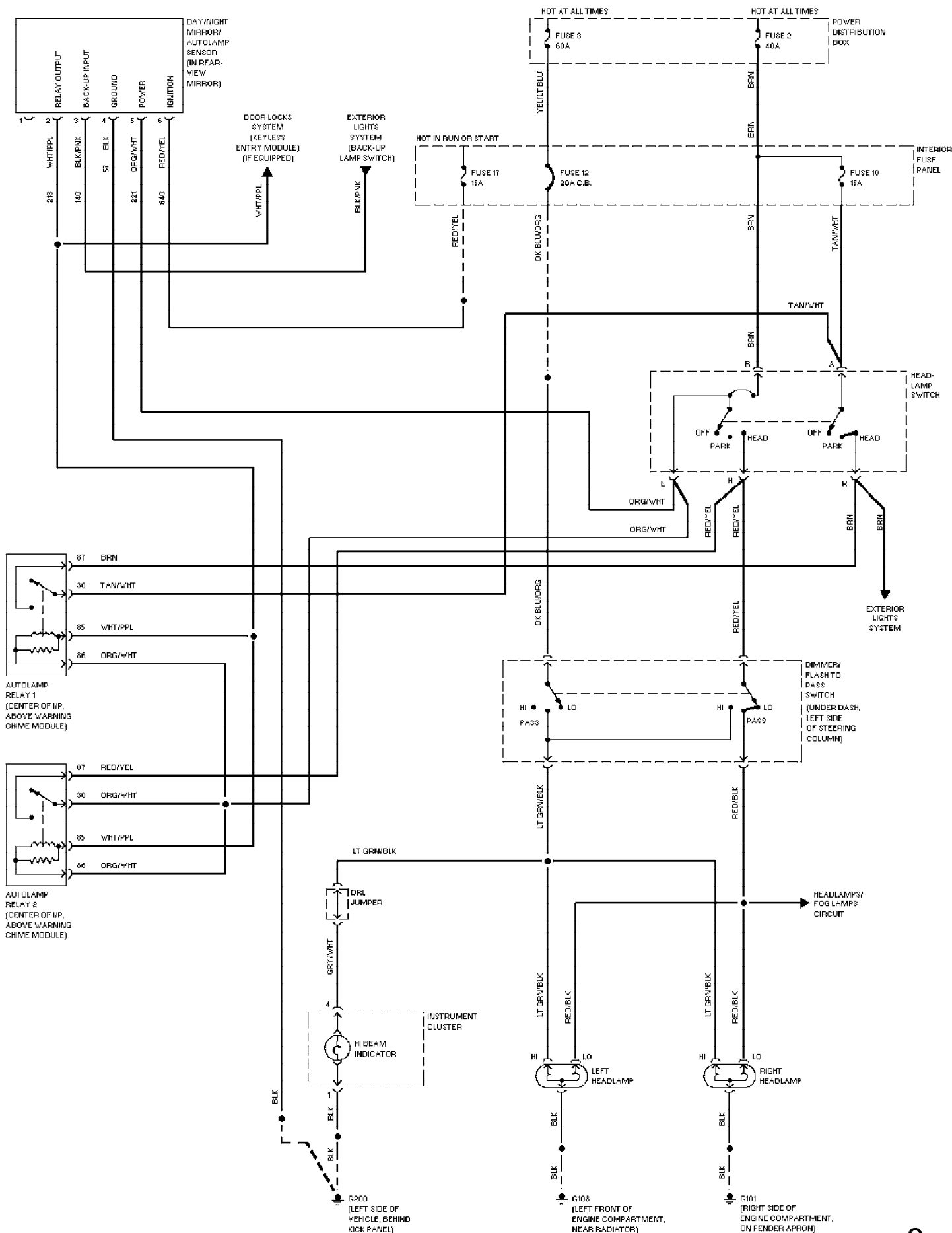
Fig. 14: Headlamps Circuit, W/ Autolamps 1994 Ford Explorer
