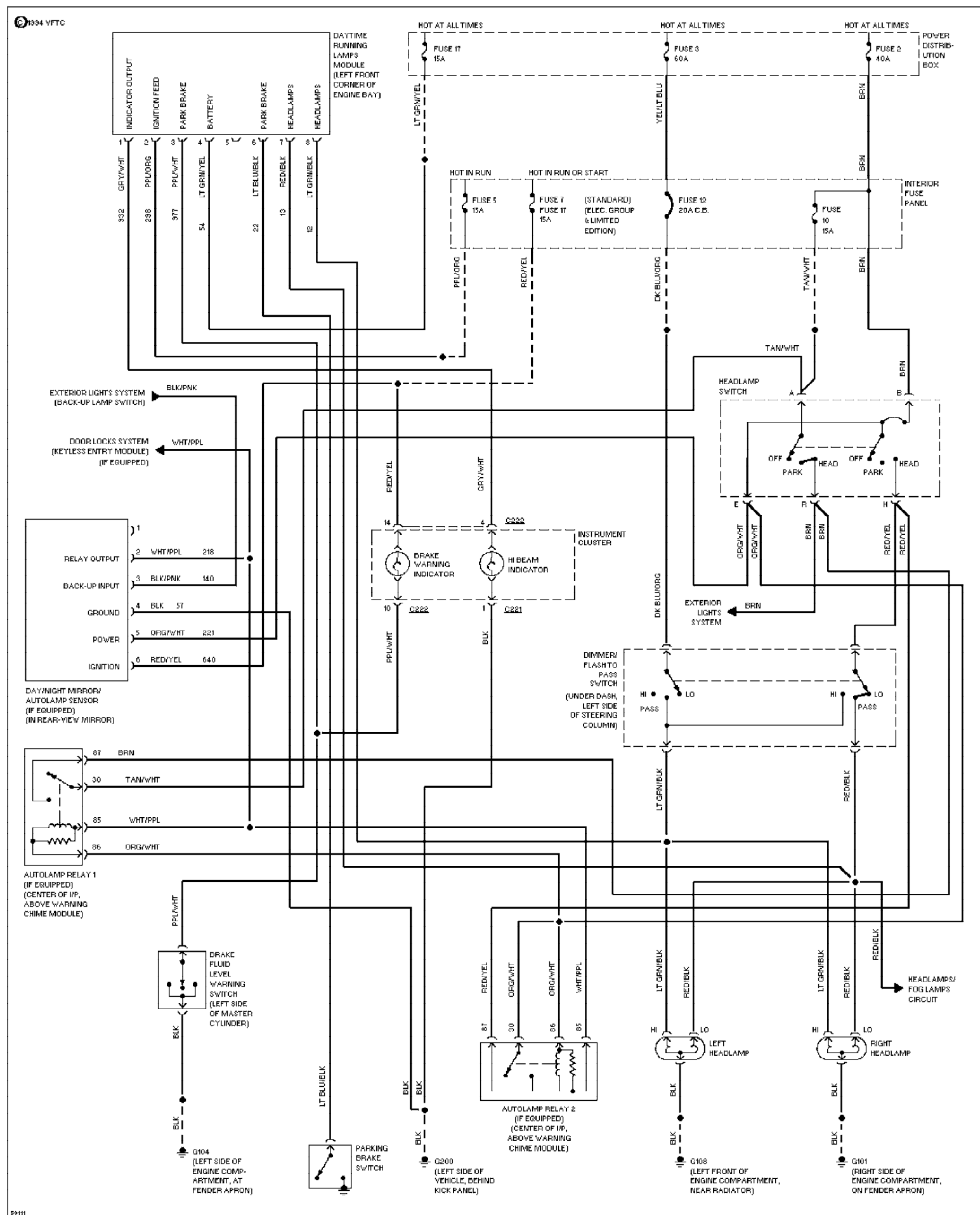
Fig. 15: Headlamps Circuit, W/ DRL 1994 Ford Explorer
