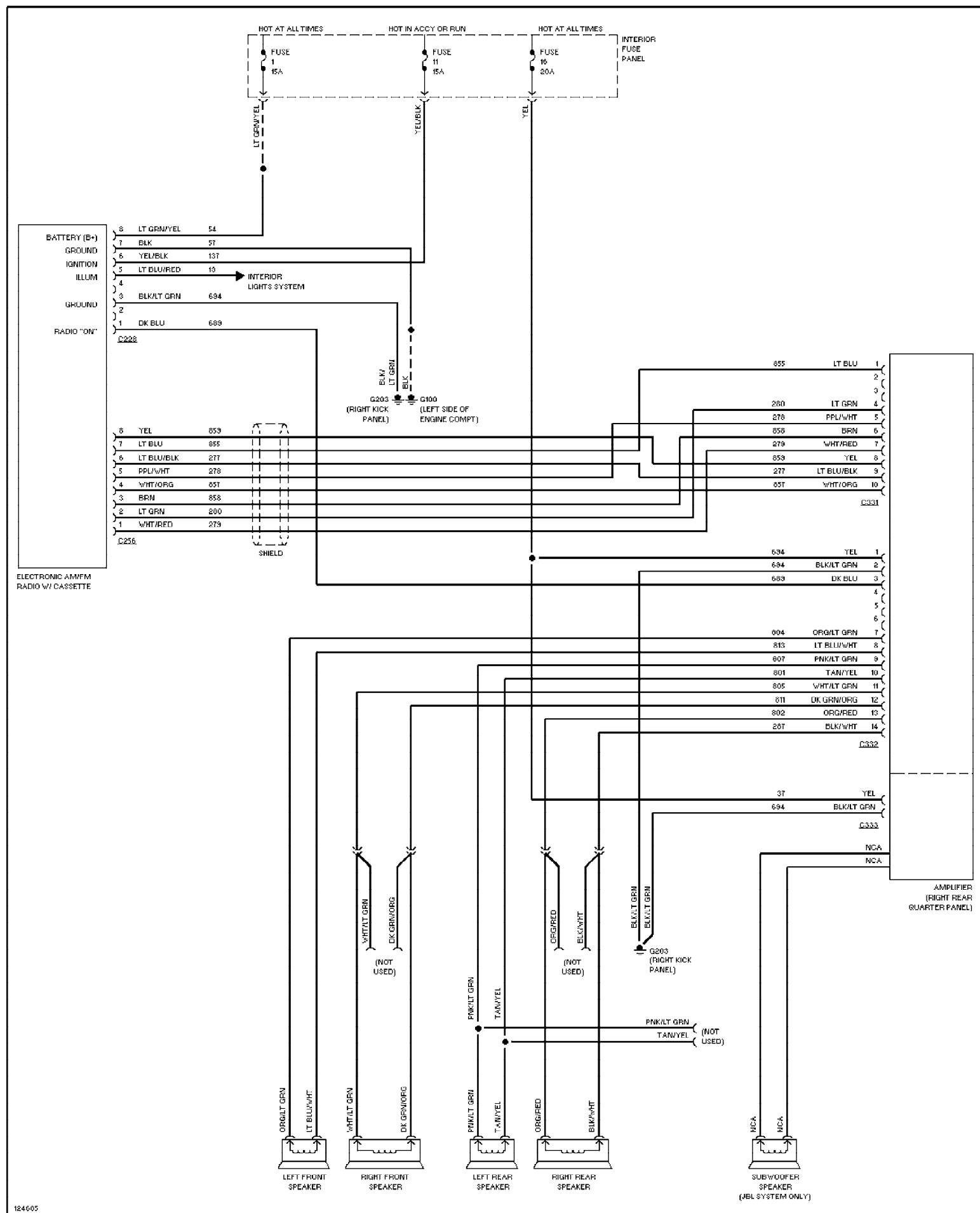
Fig. 43: Premium Sound Radio Circuit 1994 Ford Explorer
