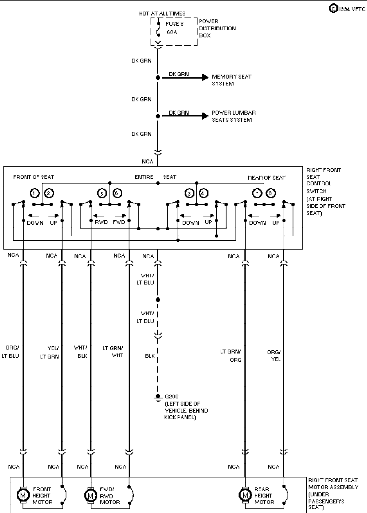
Fig. 39: Power Seat Circuit, Limited Edition 1994 Ford Explorer
