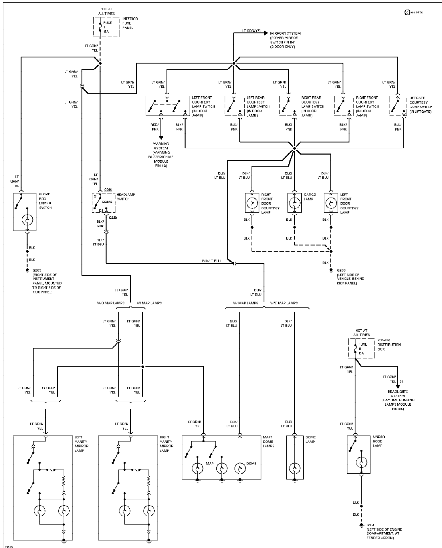
Fig. 20: Courtesy Lamps Circuit, Base 1994 Ford Explorer
