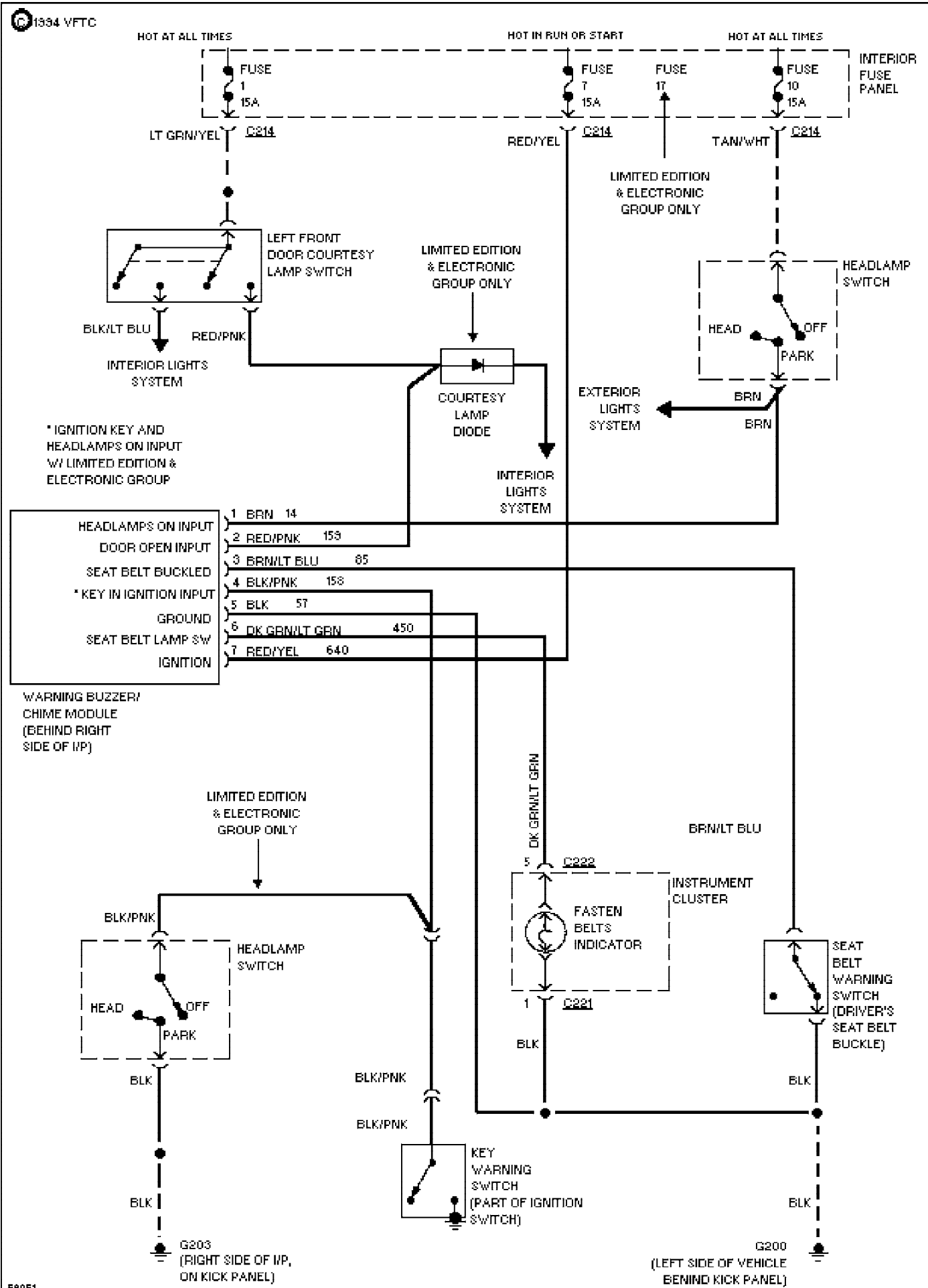
Fig. 48: Warning System Circuits 1994 Ford Explorer
