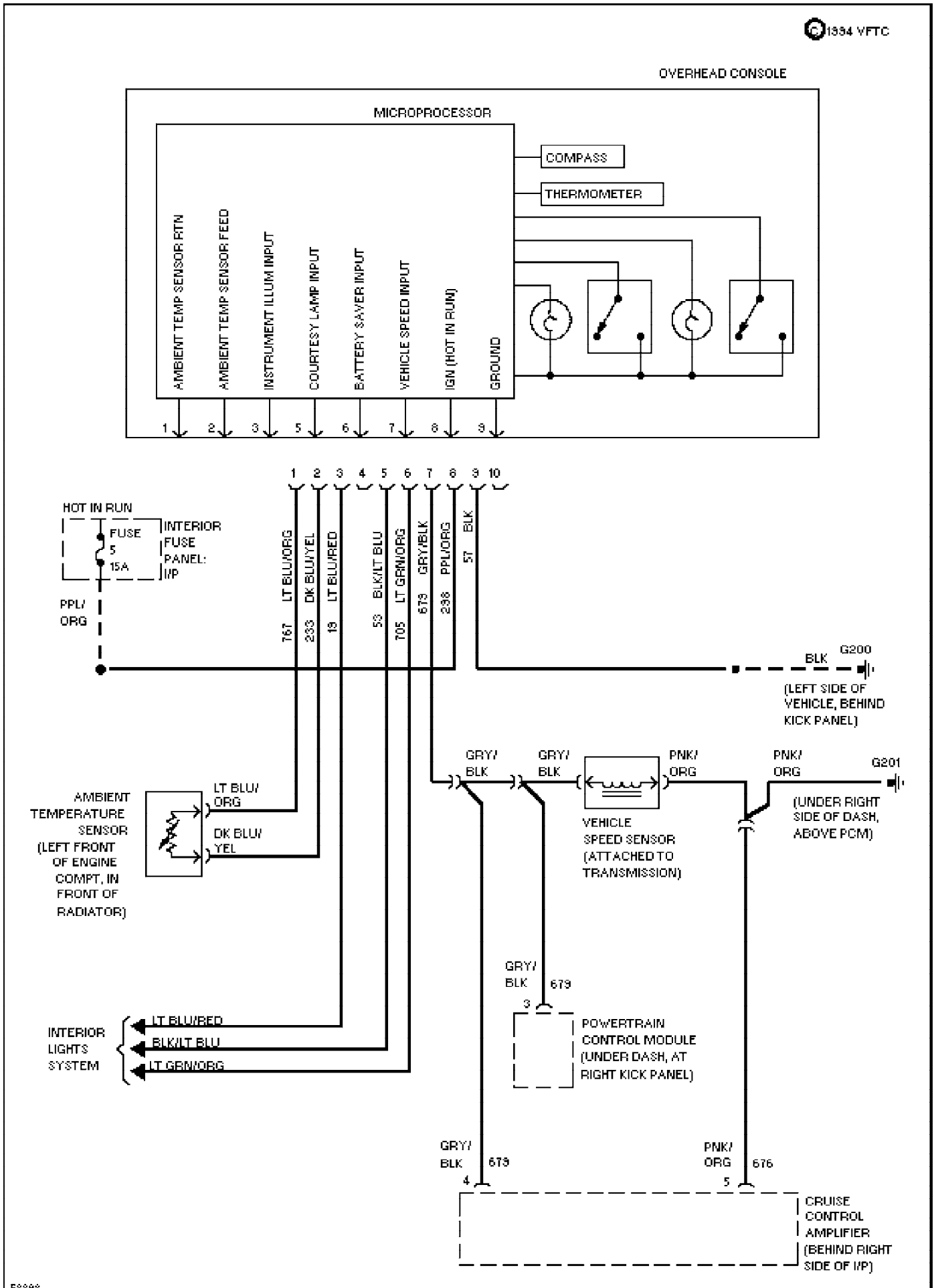
Fig. 19: Overhead Console Circuit 1994 Ford Explorer
