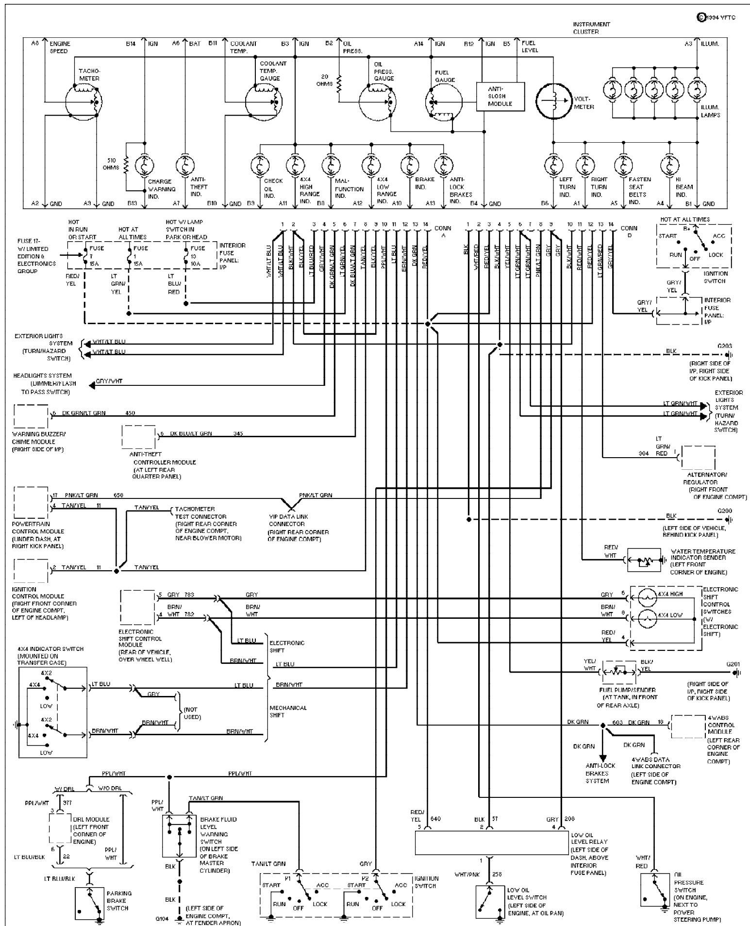
Fig. 18: Instrument Cluster Circuit 1994 Ford Explorer
