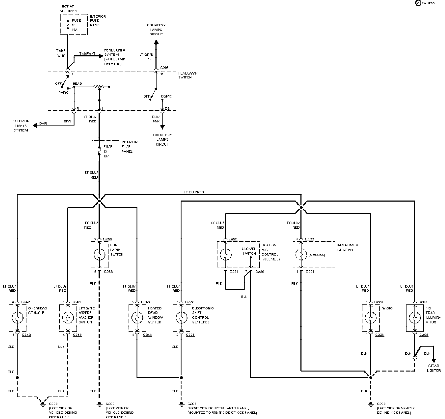
Fig. 23: Instrument Illumination Circuit, Limited Edition and Electronic Group 1994 Ford Explorer
