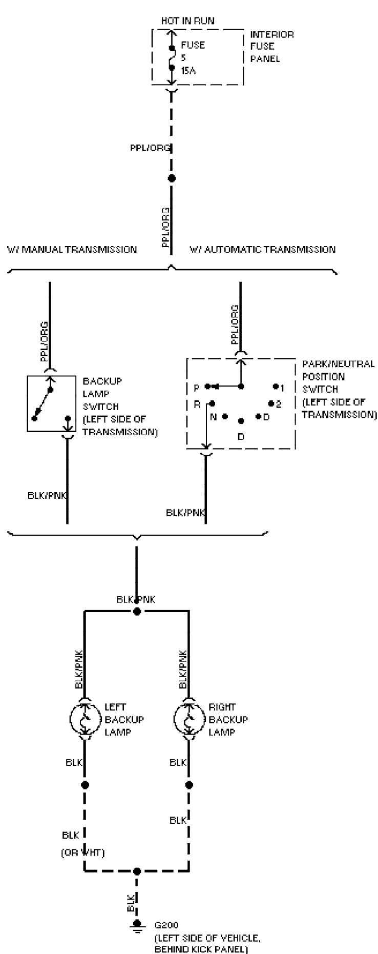
Fig. 8: Backup Lamps Circuit 1994 Ford Explorer
