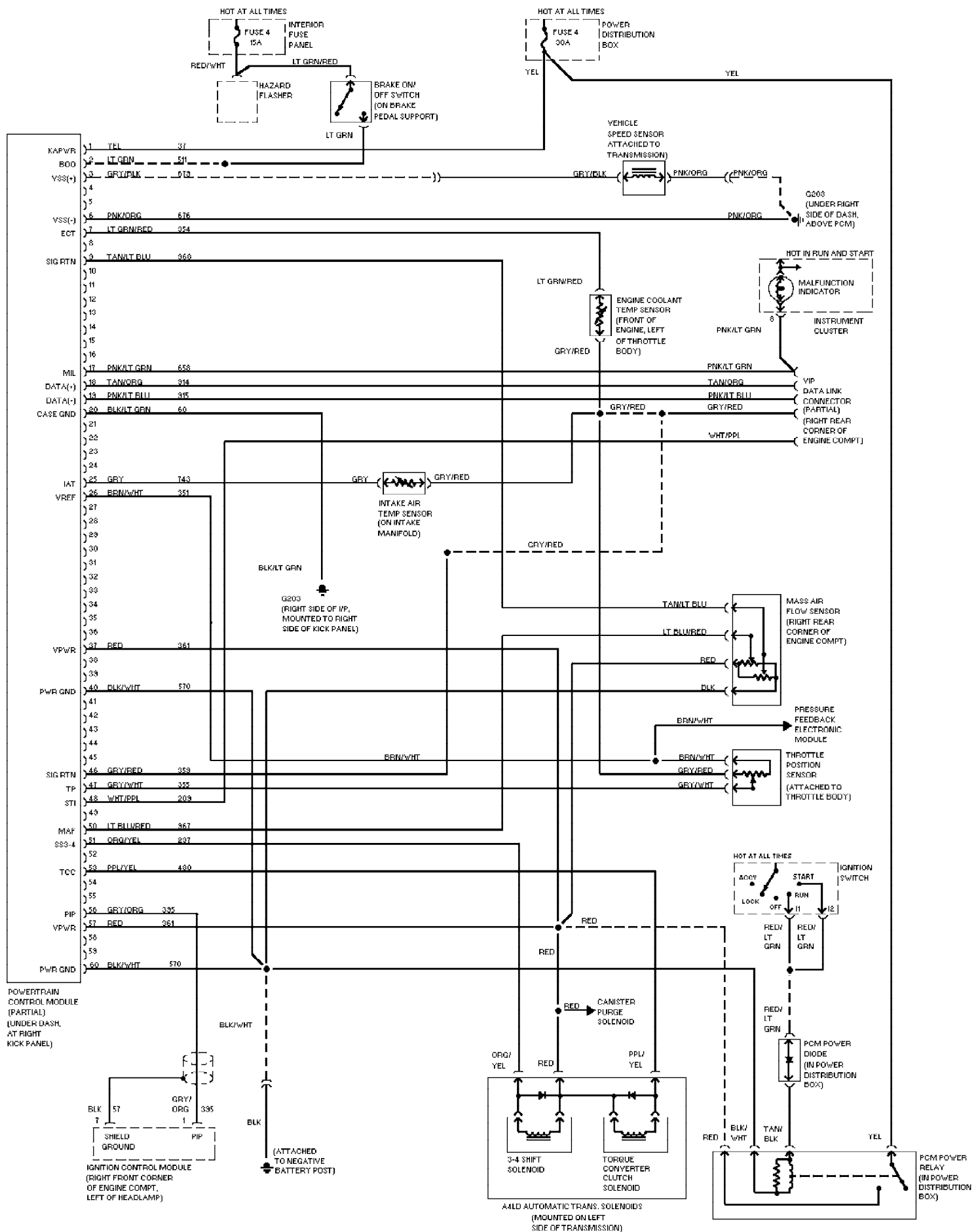
Fig. 47: 4.0L, Transmission Circuit 1994 Ford Explorer
