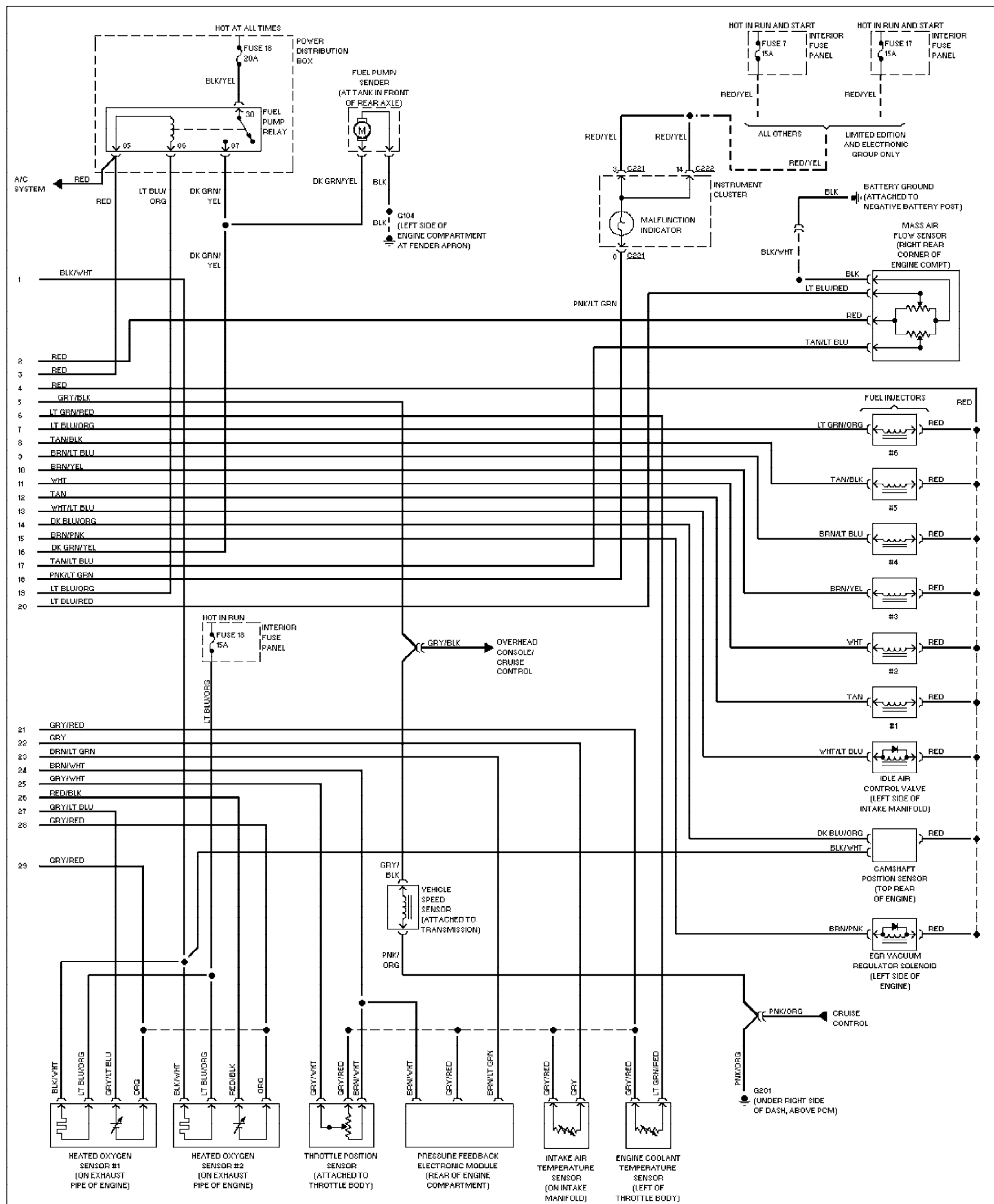
Fig. 7: 4.0L, Engine Performance Circuits (2 of 2) 1994 Ford Explorer
