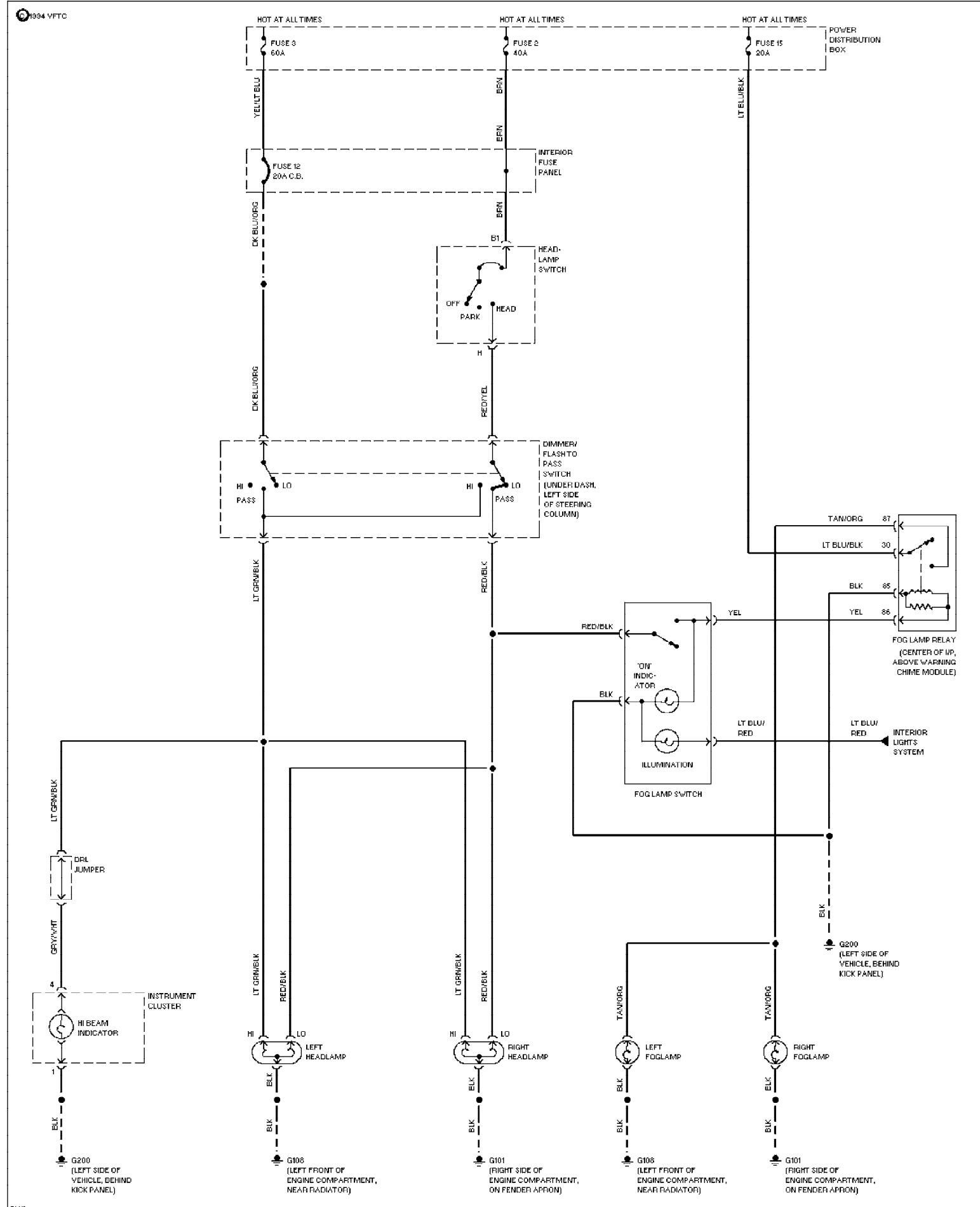
Fig. 16: Headlamps/Fog Lamps Circuit 1994 Ford Explorer
