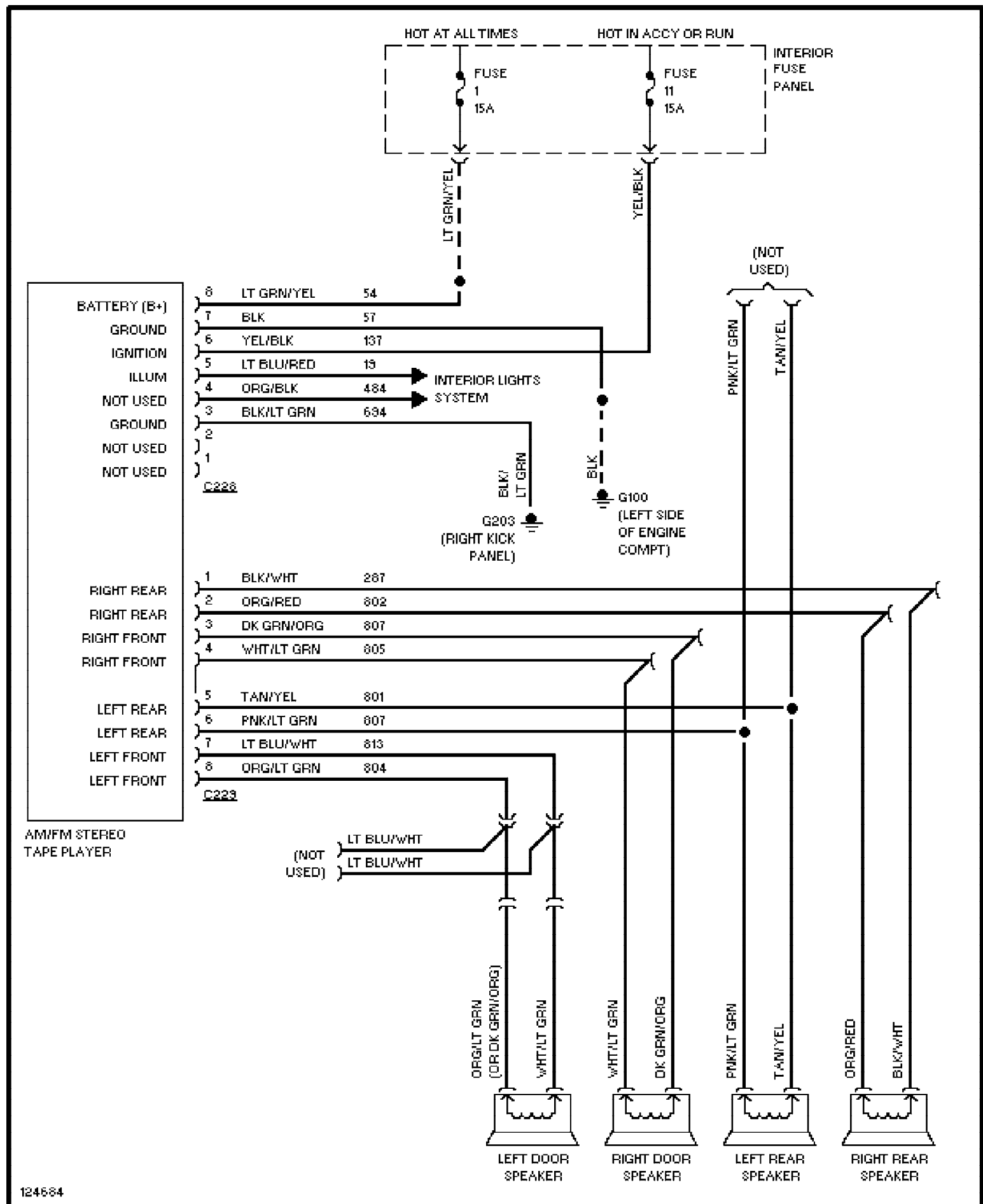
Fig. 42: Base Radio 1994 Ford Explorer
