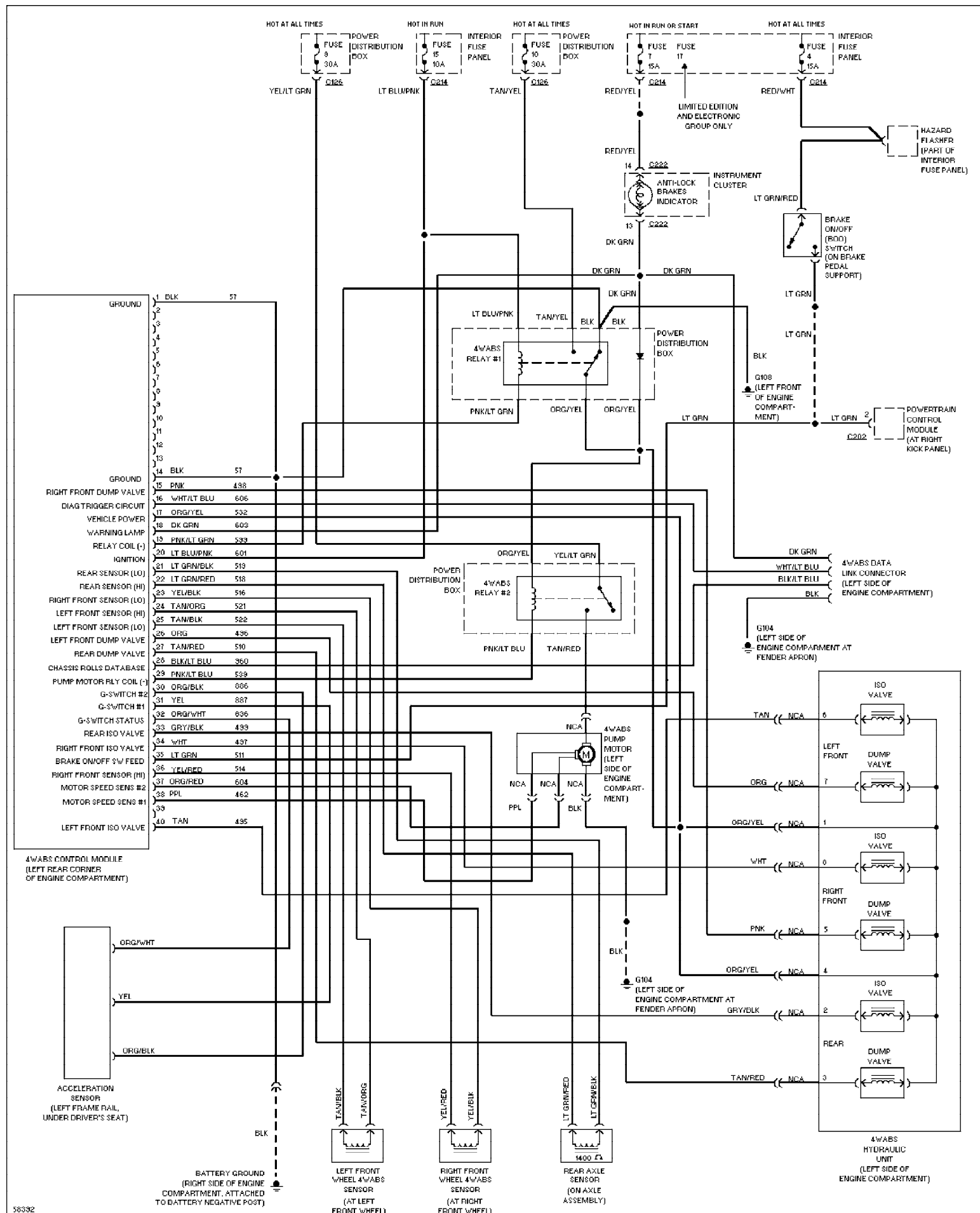
Fig. 1: Anti-lock Brake Circuits 1994 Ford Explorer
